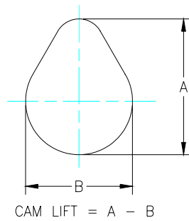
Drawing 9433064/1 CAM LIFT MEASUREMENT
