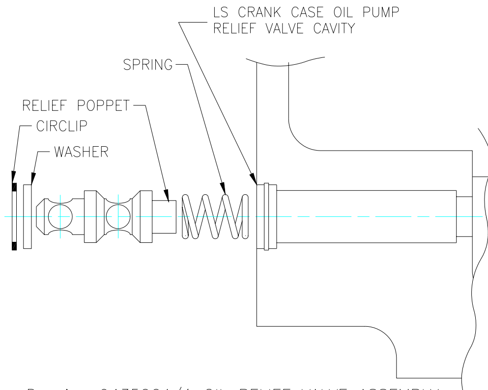
Drawing 9435064/1 OIL RELIEF VALVE ASSEMBLY
