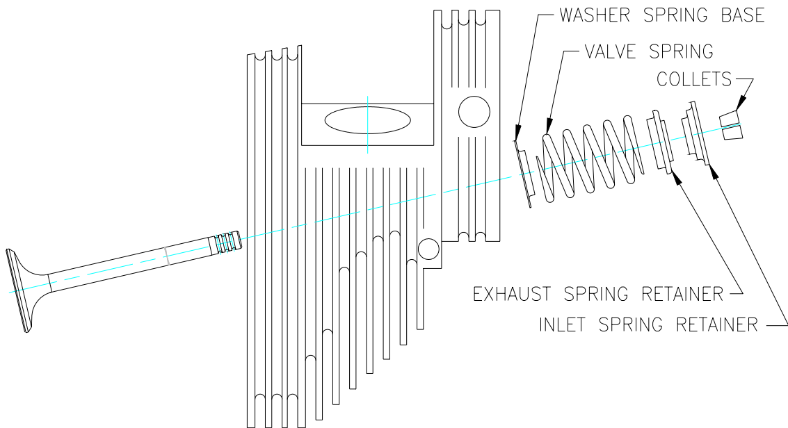
Drawing 94470641/1 VALVE ASSEMBLY
