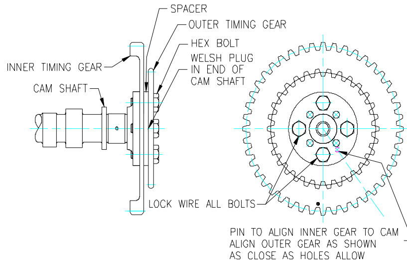
Drawing 9448064
