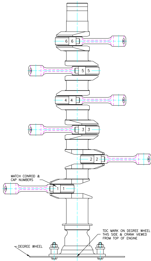
Drawing 9478083
