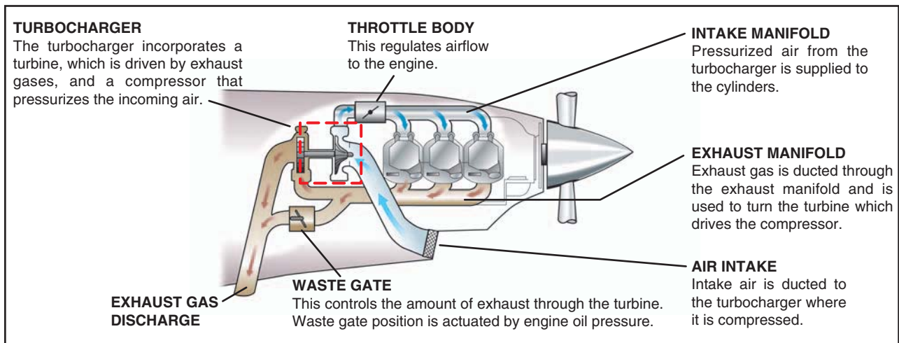
Figure 11-5. Turbocharging system.
