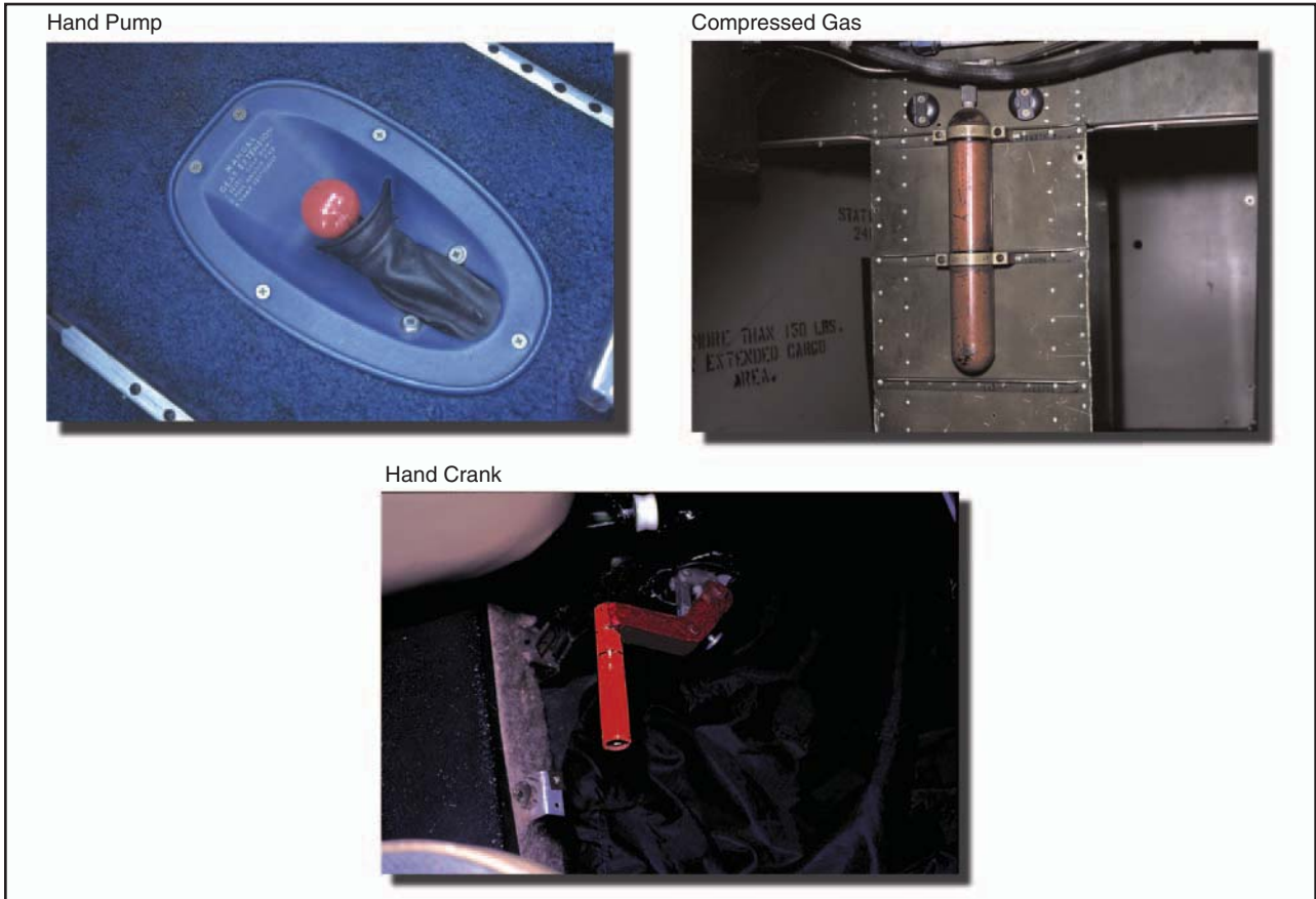
Figure 11-9. Typical emergency gear extension systems.
