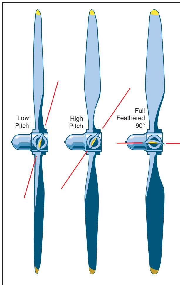
Figure 12-2. Feathered propeller.
