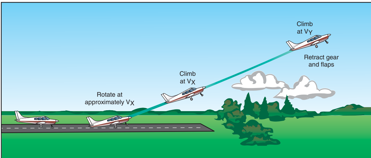
Figure 5-7. Short-field takeoff.
