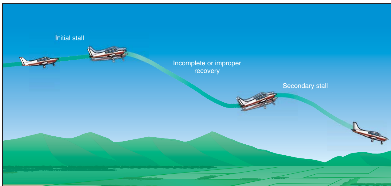
Figure 4-7. Secondary stall.
