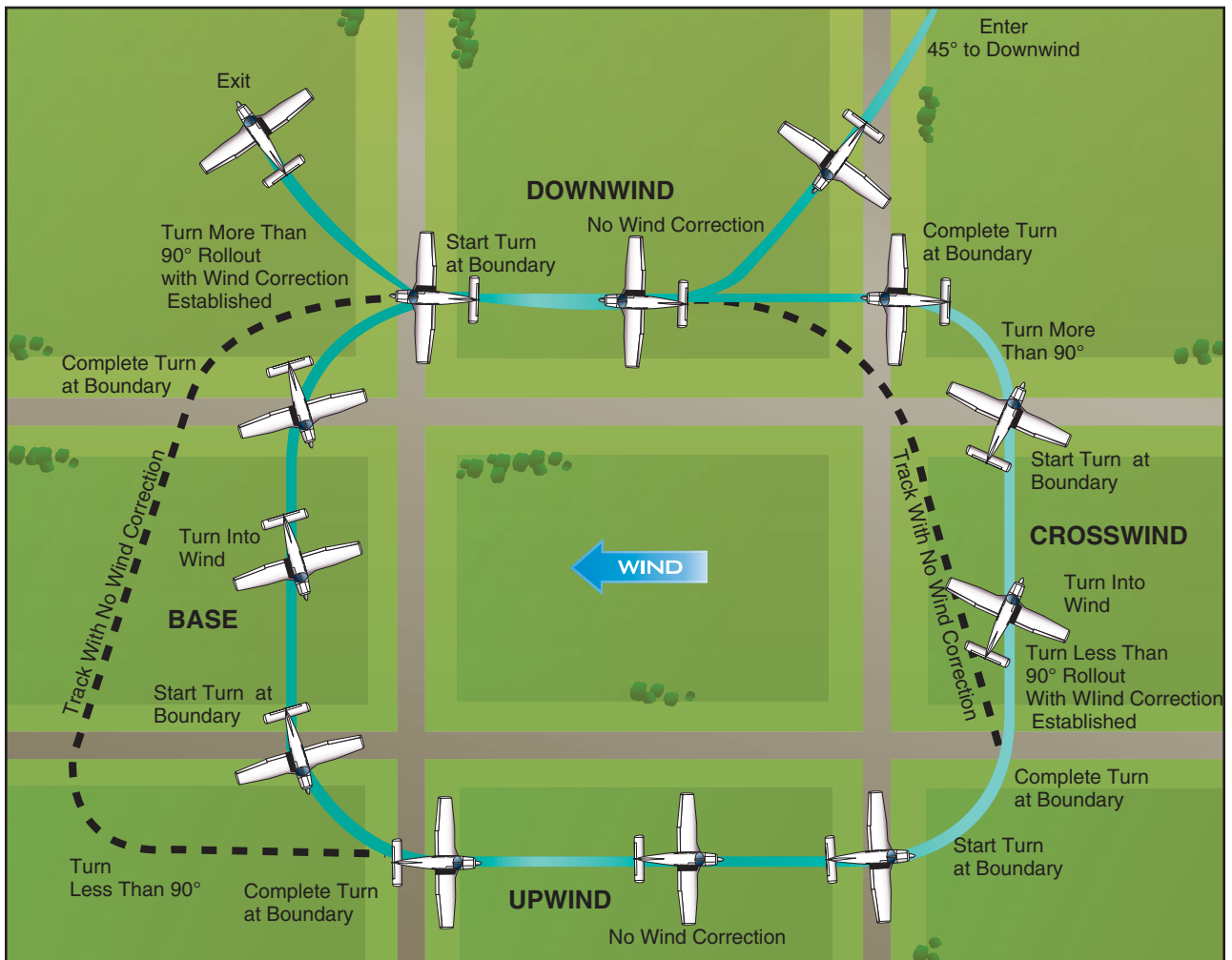
Figure 6-4. Rectangular course.
