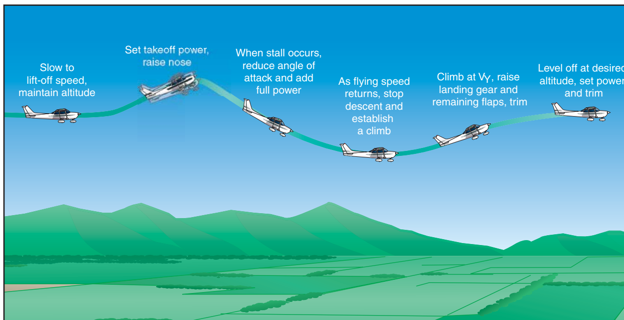
Figure 4-6. Power-on stall.
