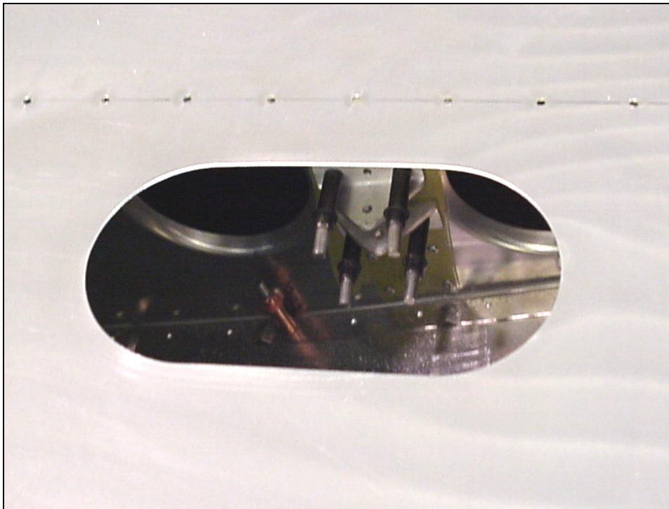
Aileron bellcrank access hole in rear bottom skin.
