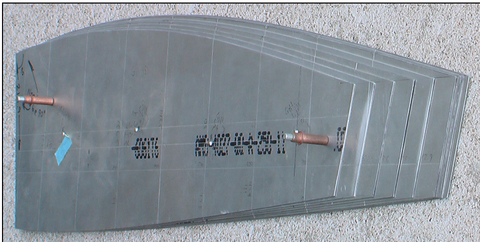
Photo of the XL rear rib blanks (1 through 9) stack together (for illustration purposes).
