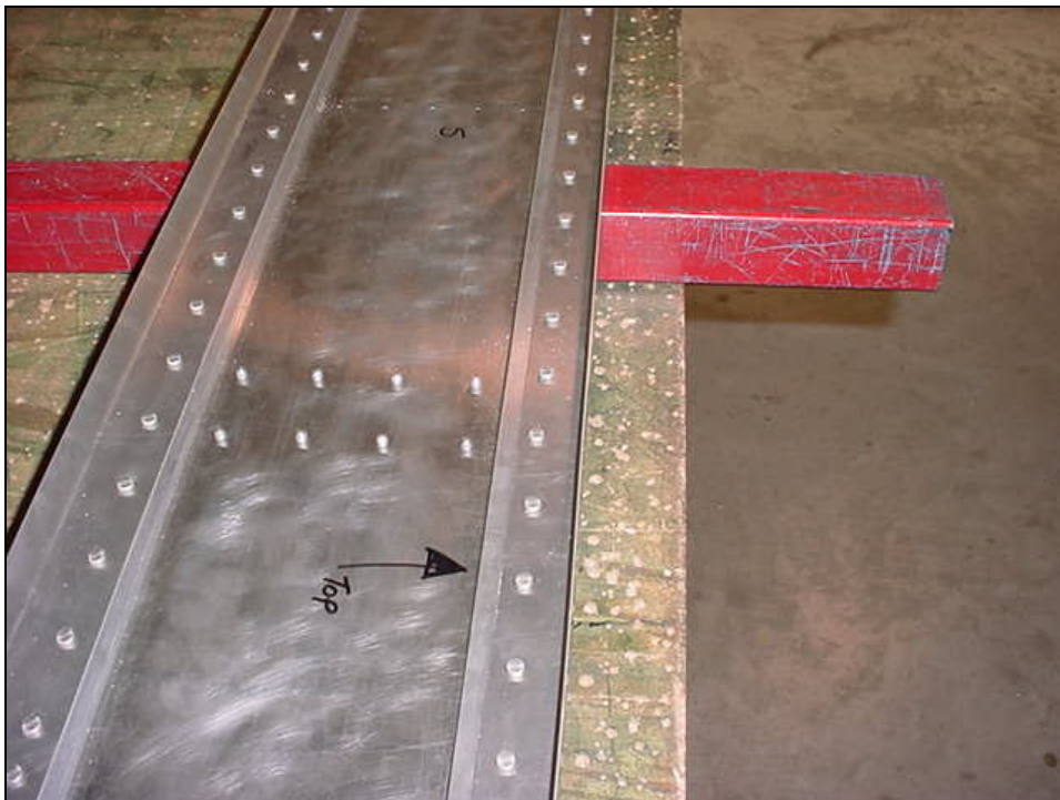
MARK: Identify the top side of the spar, and mark an arrow TOP (top spar cap angle 6W3-6 has the flange bend 90 degrees).
