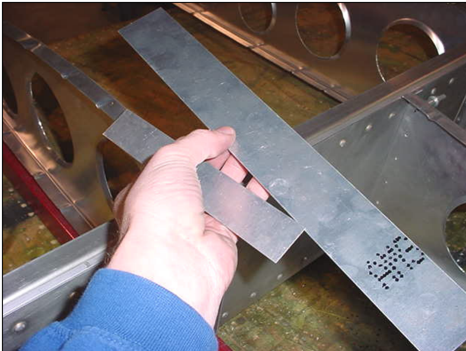
.025" strip top flange of cap angle 6W3-8
