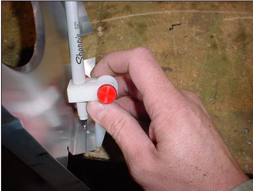
Edge marker block (adjustable) P/N 6352
