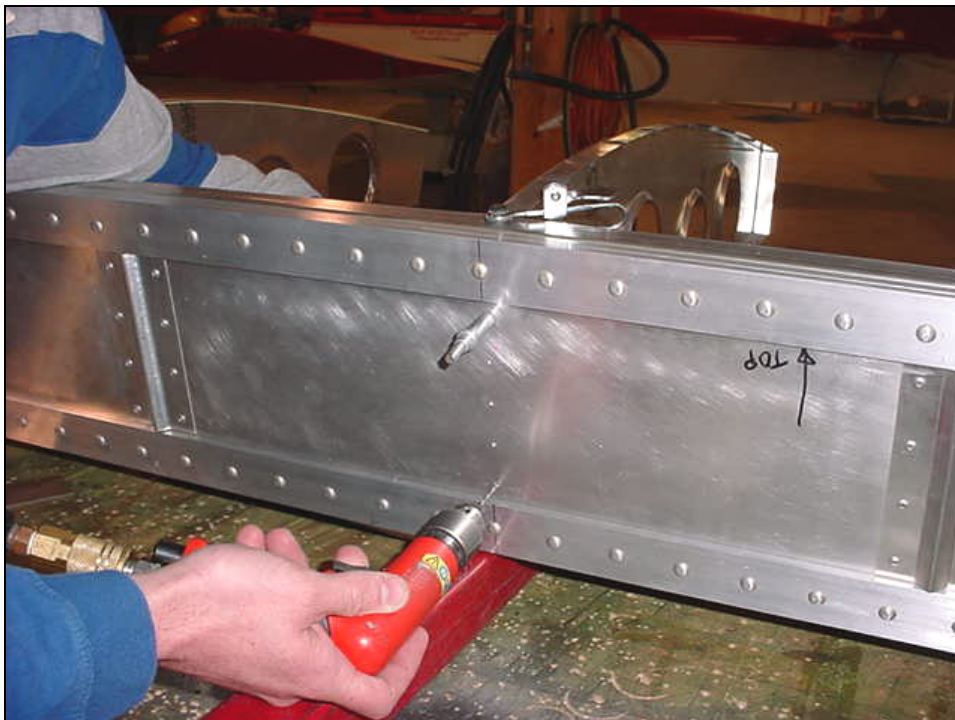
All the rear ribs are square to the top flange of the spar.
