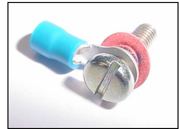
Ring terminal (ground) over paper washer.
