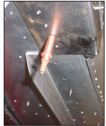
Bottom rivet line through the Floor Channel 6TD3-2 A5 PITCH 30
