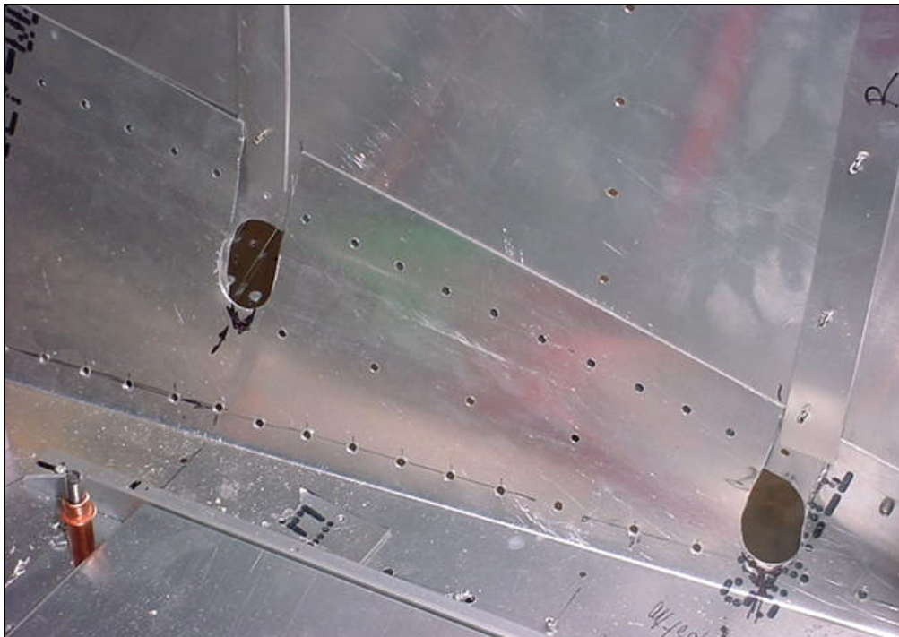
Inside view of right side. Cutout in Cabin Floor Skin 6B10-1, cutout to make room for the tube.
