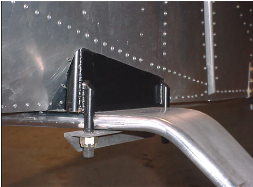
Cutout in the side skin is below the diagonal rivet line.
