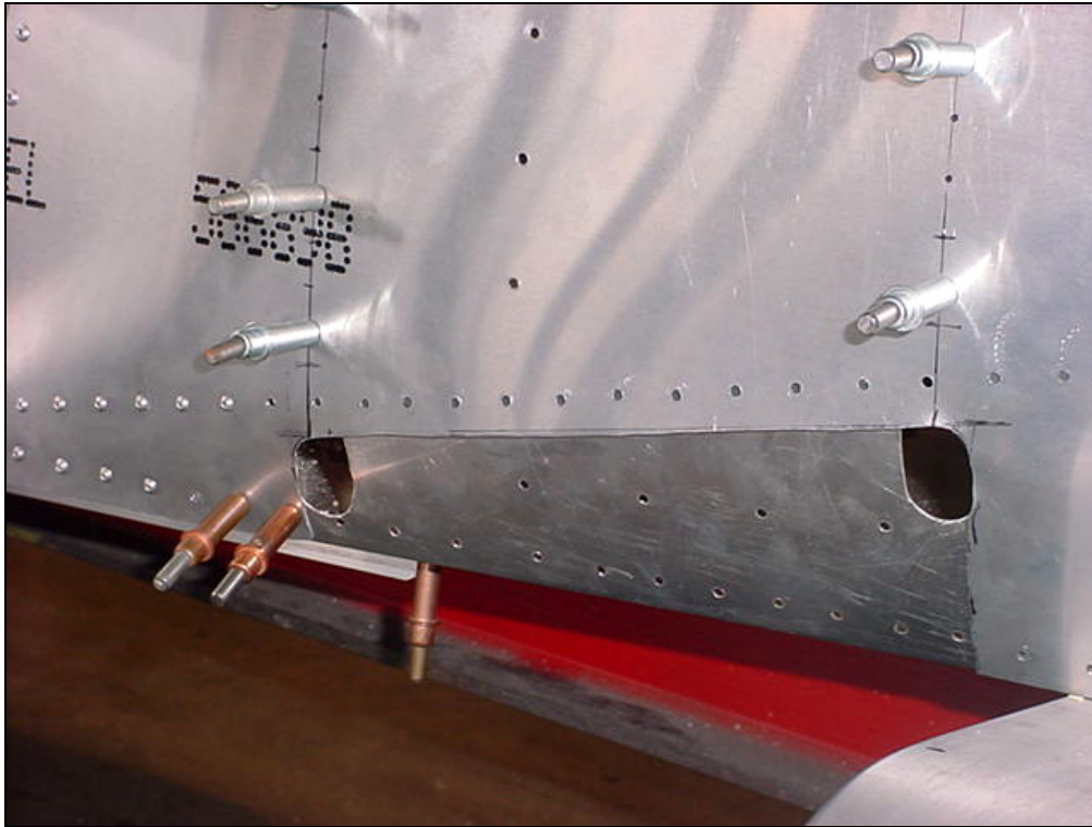
Rectangular cutout in the fuselage Forward Side Skin 6B11-2
