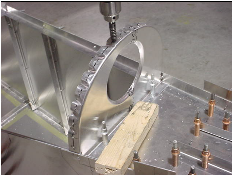
Baggage back bulkhead.
