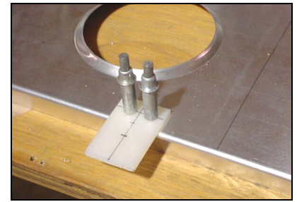
N66 PLASTIC FAIRLEAD 2 RIVETS A5
