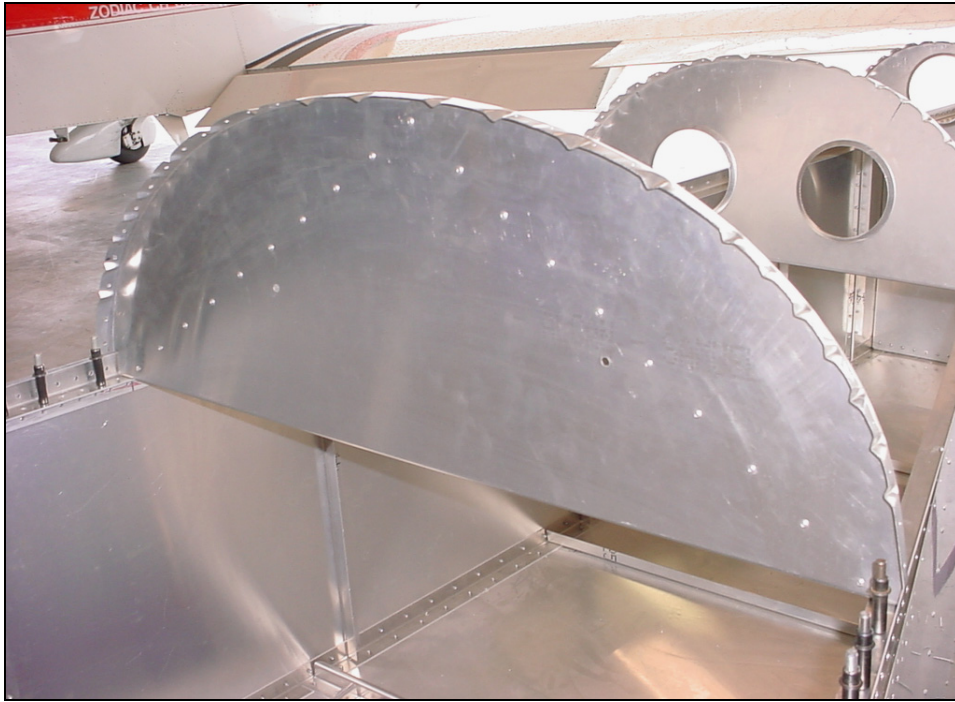
Baggage back bulkhead.
