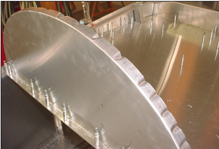
31 PILOT HOLES IN 6B12-2
