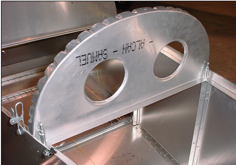
MIDDLE BULKHEAD 6B12-1
