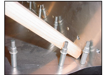
Bottom detail. Support in corner of spar with cabin floor.
