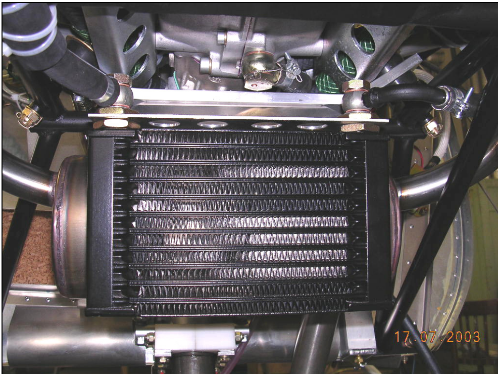
Oil cooler bracket bolted to rear Dynafocal Bracket E2-1X
