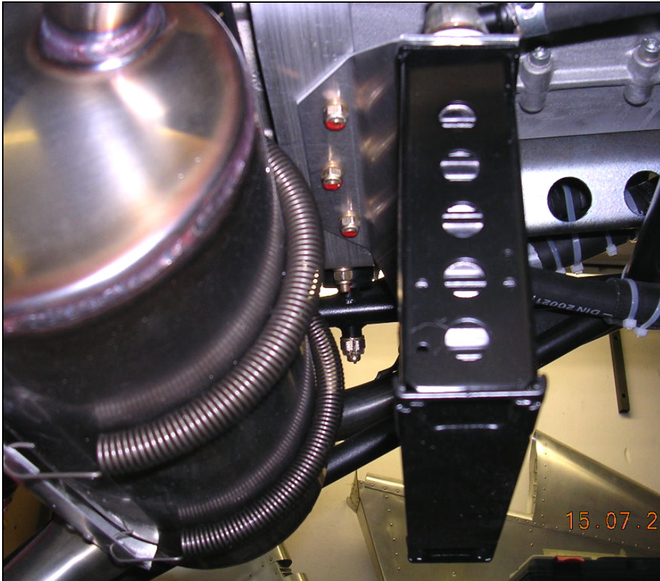
Oil cooler bracket bolted to rear Dynafocal Bracket E2-1X
