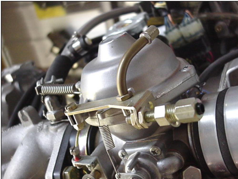
Remove the cable adjuster on the carburetor, open the hole in the mounting bracket and crew in the cable stop adjuster 25-0700
